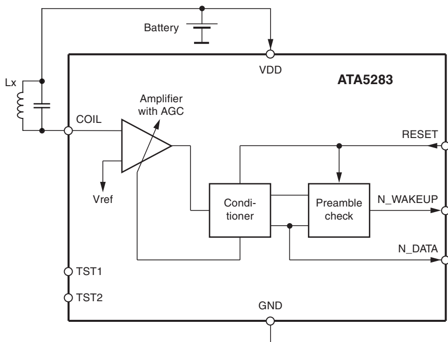
Figure 1-1. Block Diagram
